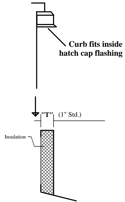
Section view of hatch sleeving into curb
